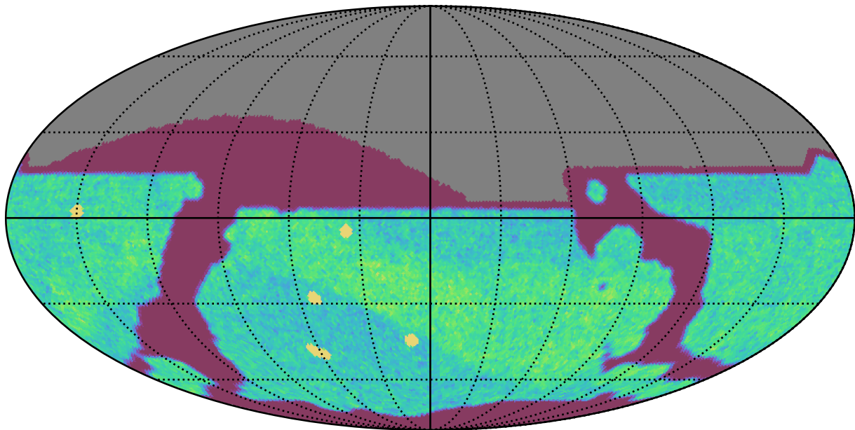
too_elab_r16_d2_giz_v3.4_10yrs All sky i band: NVisits
