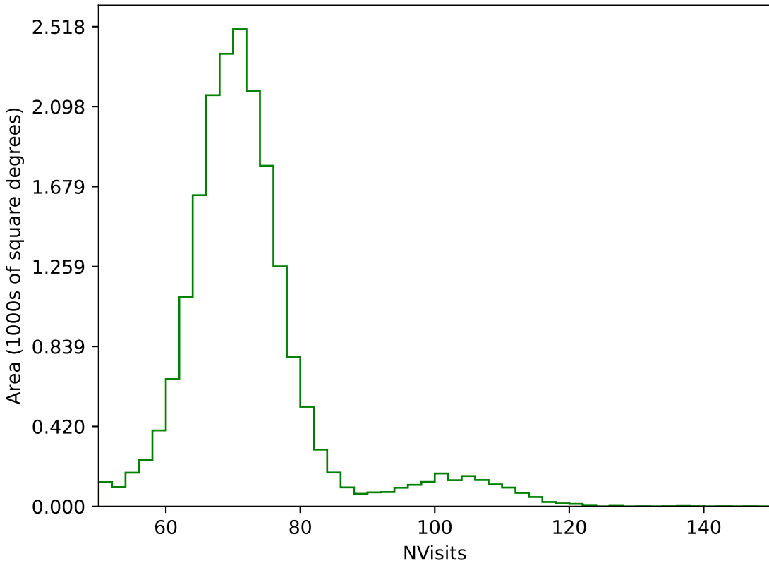
too_elab_r16_d2_giz_v3.4_10yrs All sky g band: NVisits
