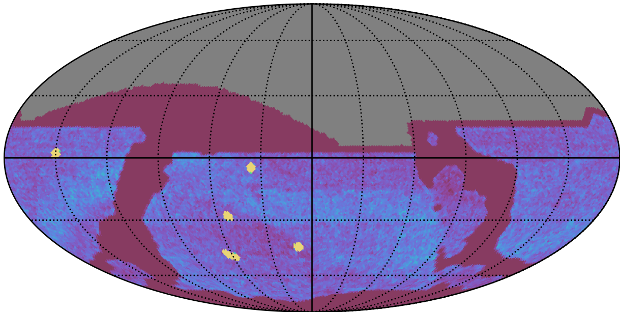
too_elab_r16_d2_giz_v3.4_10yrs All sky all bands: NVisits
