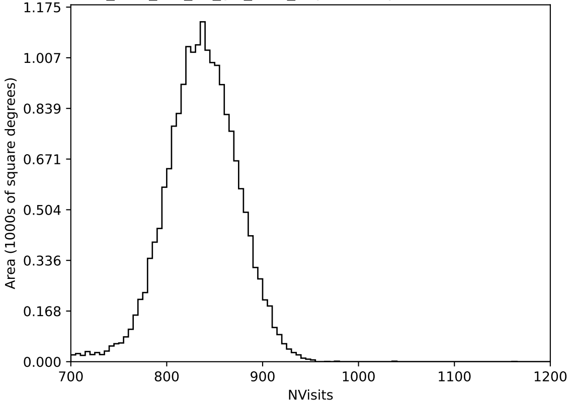
too_elab_r16_d2_giz_v3.4_10yrs All sky all bands: NVisits
