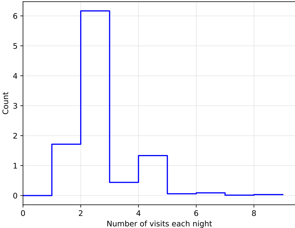
too_elab_r16_d2_giz_v3.4_10yrs All sky: NVisitsPerNight
