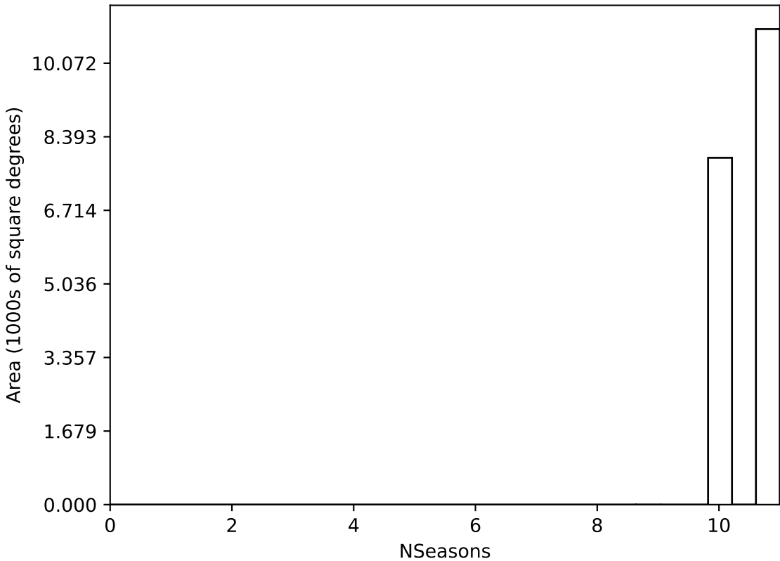
too_elab_r16_d2_giz_v3.4_10yrs WFD all bands: NSeasons
