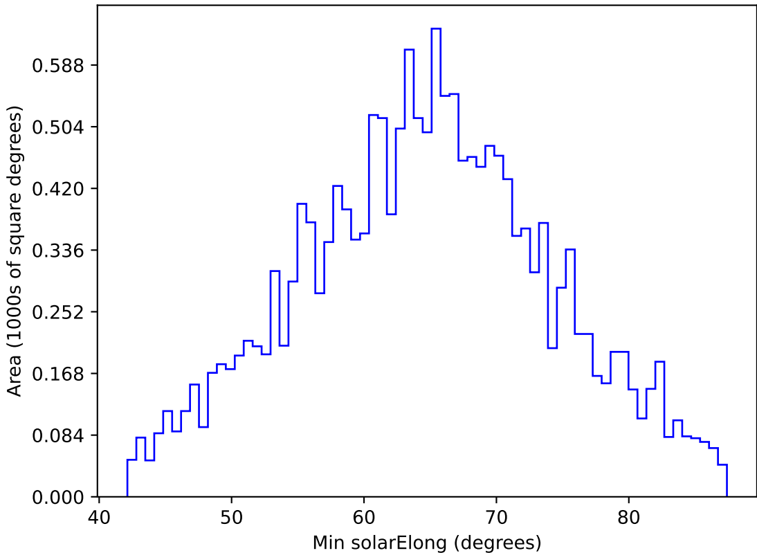
too_elab_r16_d2_giz_v3.4_10yrs WFD y band: Min solarElong
