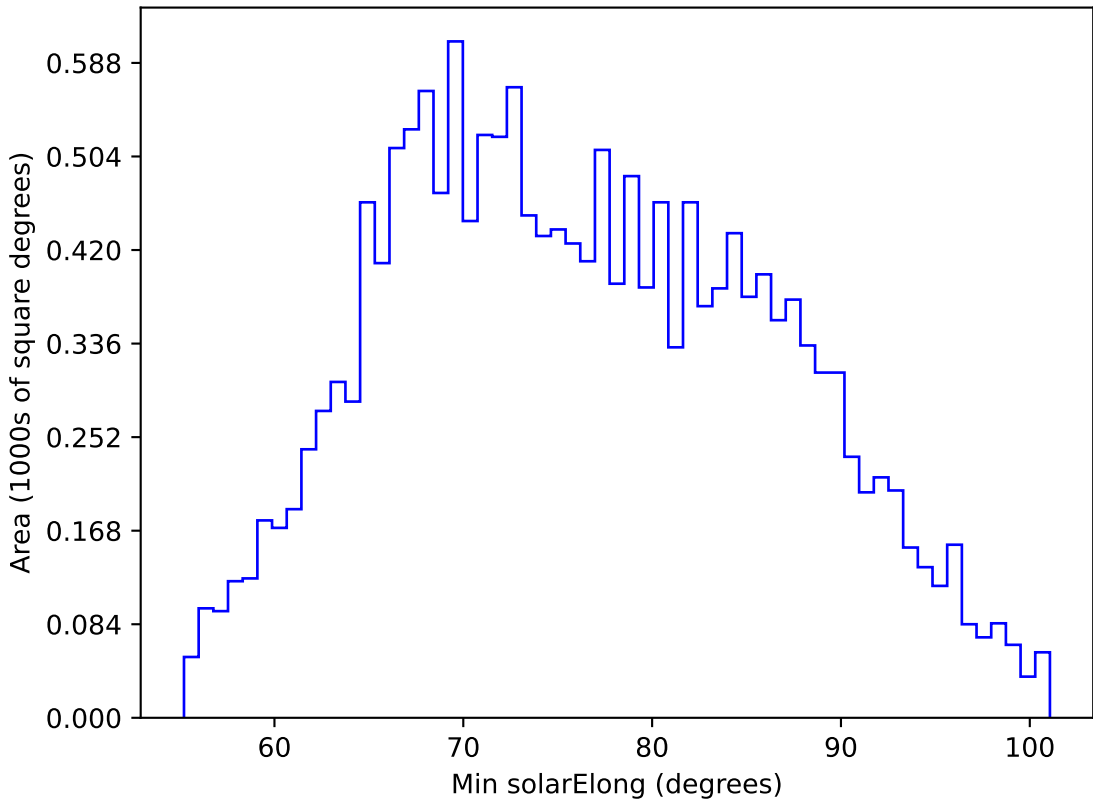
too_elab_r16_d2_giz_v3.4_10yrs WFD u band: Min solarElong
