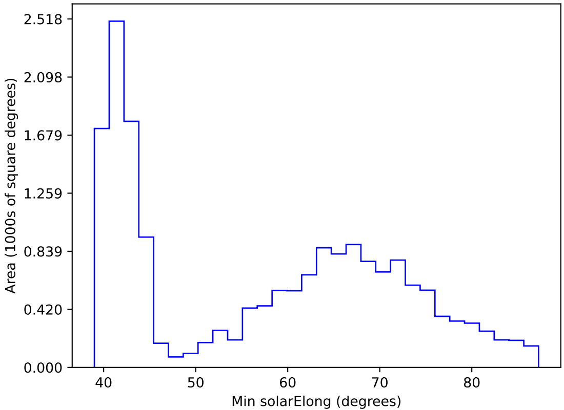
too_elab_r16_d2_giz_v3.4_10yrs WFD r band: Min solarElong
