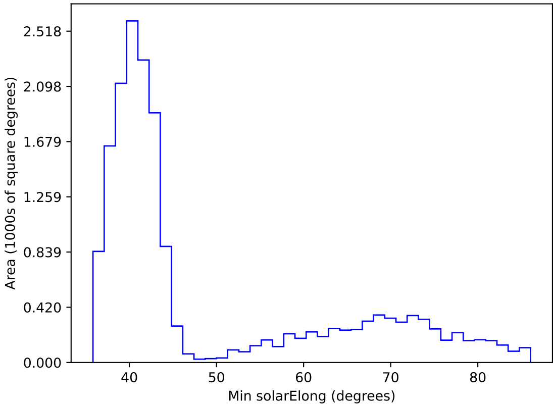
too_elab_r16_d2_giz_v3.4_10yrs WFD i band: Min solarElong
