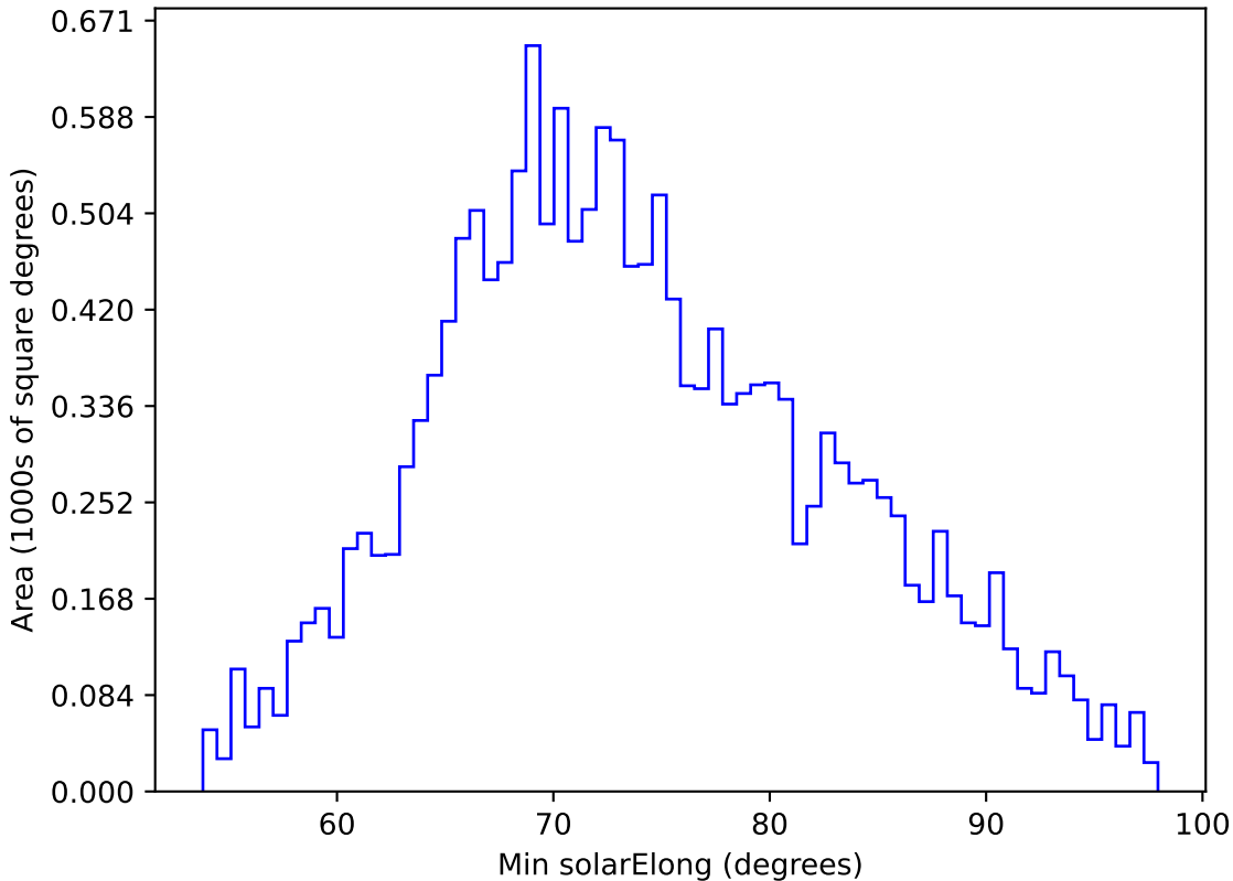
too_elab_r16_d2_giz_v3.4_10yrs WFD g band: Min solarElong
