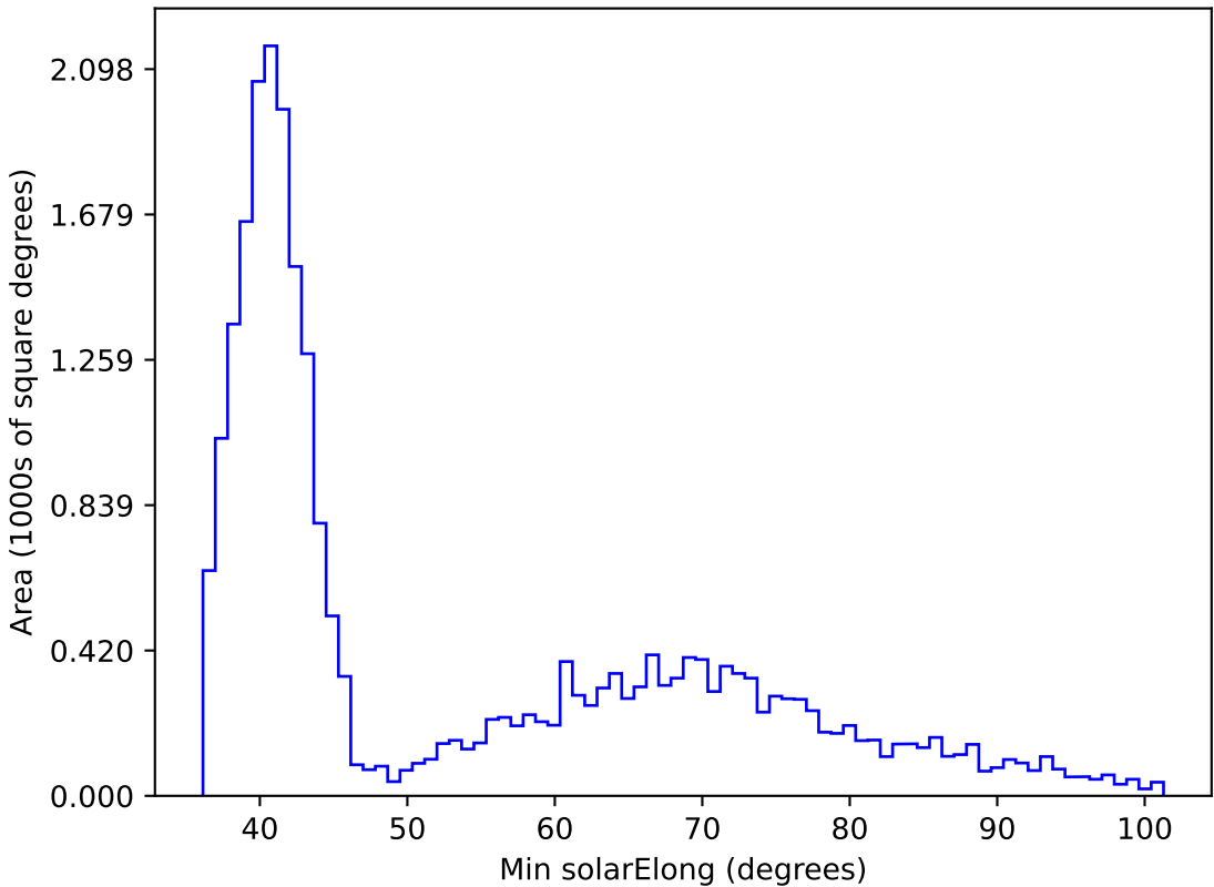
too_elab_r16_d2_giz_v3.4_10yrs All sky z band: Min solarElong
