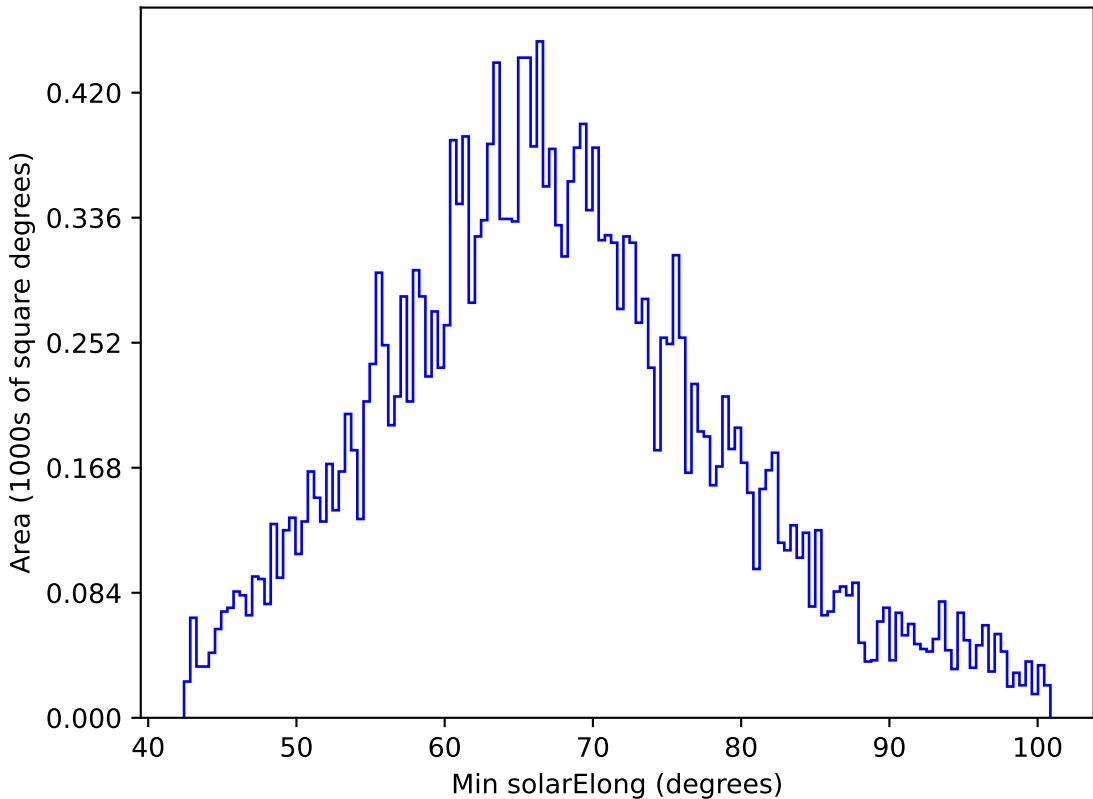
too_elab_r16_d2_giz_v3.4_10yrs All sky y band: Min solarElong
