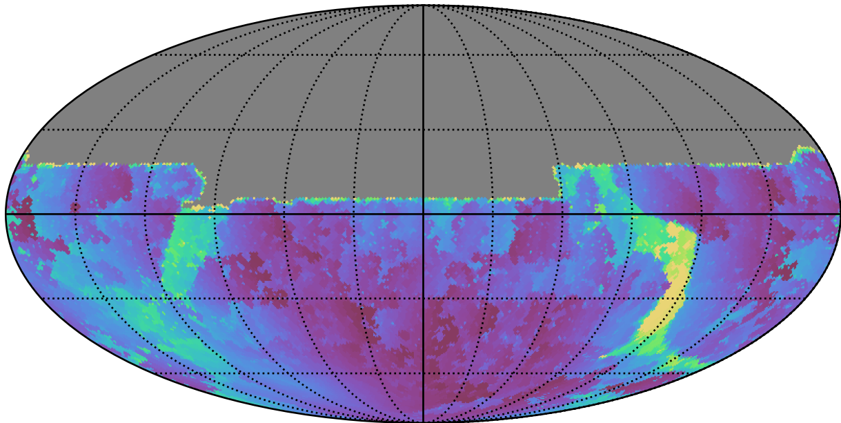
too_elab_r16_d2_giz_v3.4_10yrs All sky u band: Min solarElong
