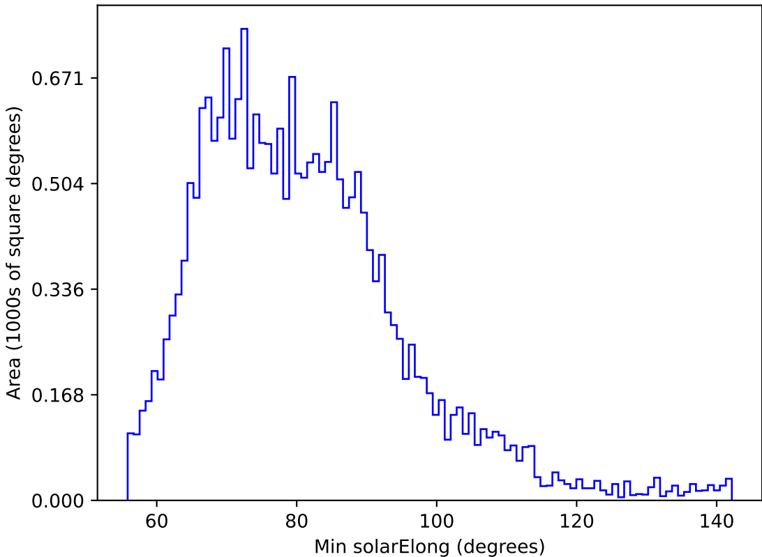
too_elab_r16_d2_giz_v3.4_10yrs All sky u band: Min solarElong
