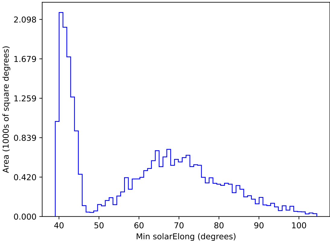
too_elab_r16_d2_giz_v3.4_10yrs All sky r band: Min solarElong
