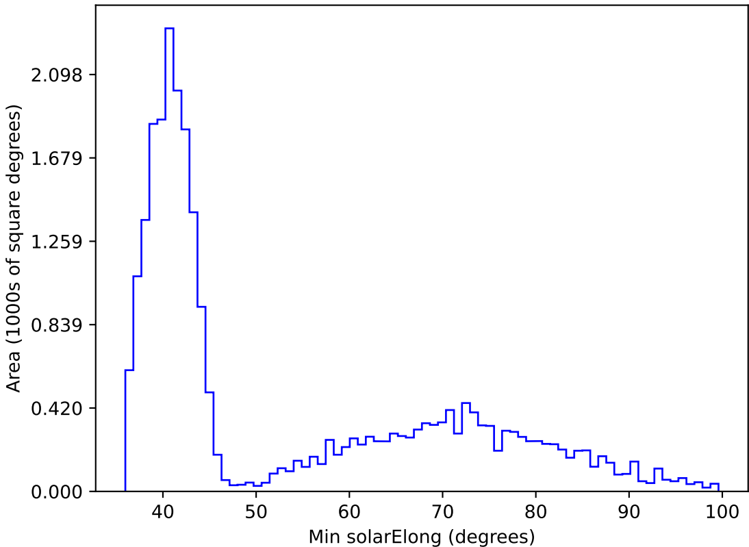
too_elab_r16_d2_giz_v3.4_10yrs All sky i band: Min solarElong
