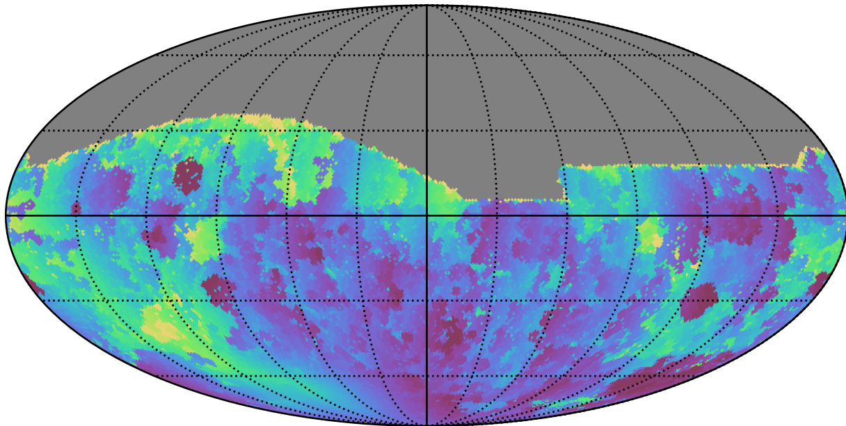
too_elab_r16_d2_giz_v3.4_10yrs All sky g band: Min solarElong
