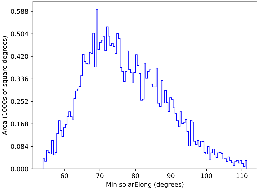
too_elab_r16_d2_giz_v3.4_10yrs All sky g band: Min solarElong
