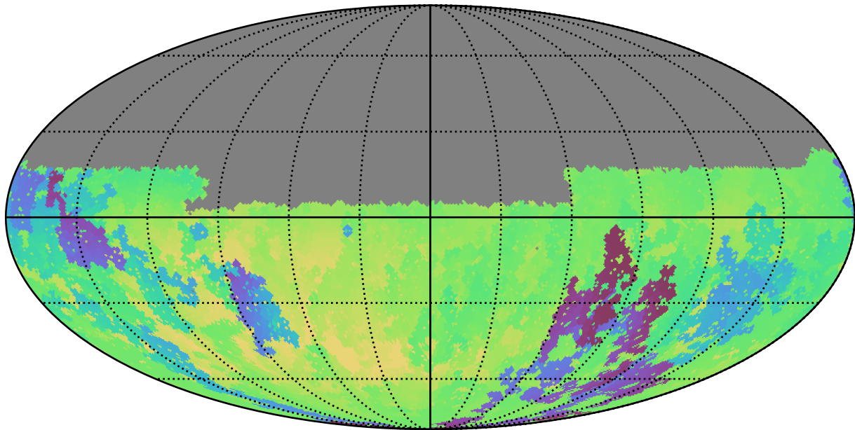
too_elab_r16_d2_giz_v3.4_10yrs Yr 1 u band: Min skyBrightness
