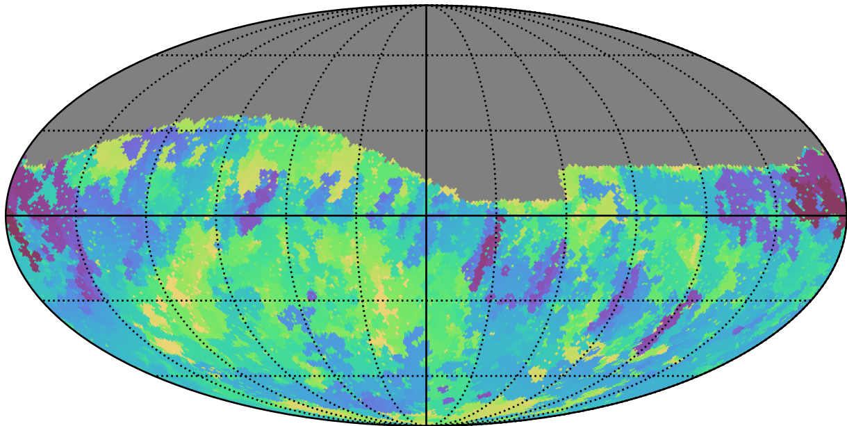
too_elab_r16_d2_giz_v3.4_10yrs Yr 1 r band: Min skyBrightness
