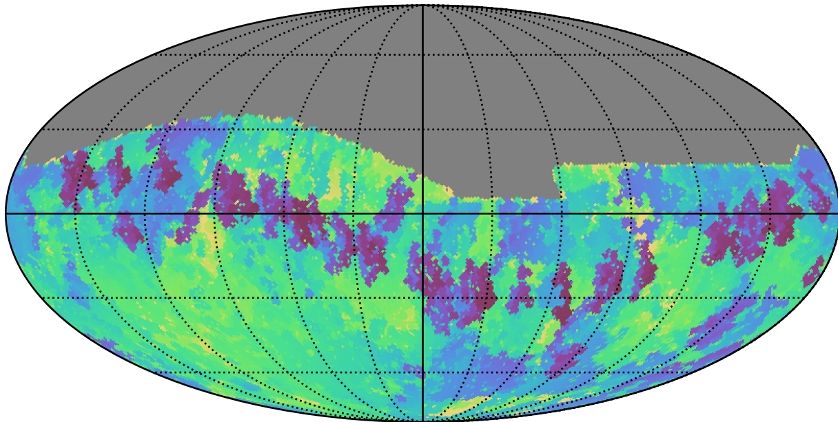
too_elab_r16_d2_giz_v3.4_10yrs Yr 1 i band: Min skyBrightness
