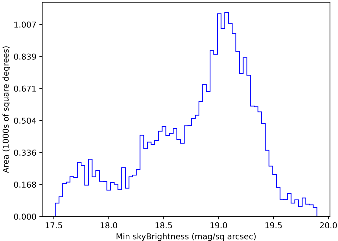
too_elab_r16_d2_giz_v3.4_10yrs Yr 1 i band: Min skyBrightness
