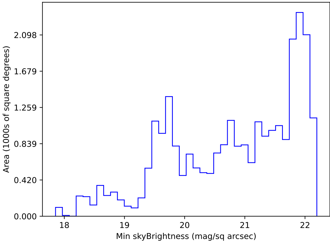
too_elab_r16_d2_giz_v3.4_10yrs Yr 1 g band: Min skyBrightness
