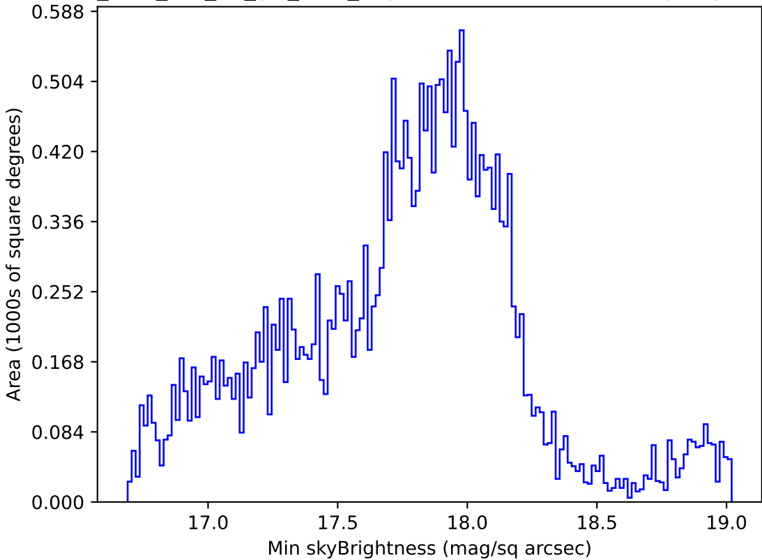
too_elab_r16_d2_giz_v3.4_10yrs Yr 1 all bands: Min skyBrightness
