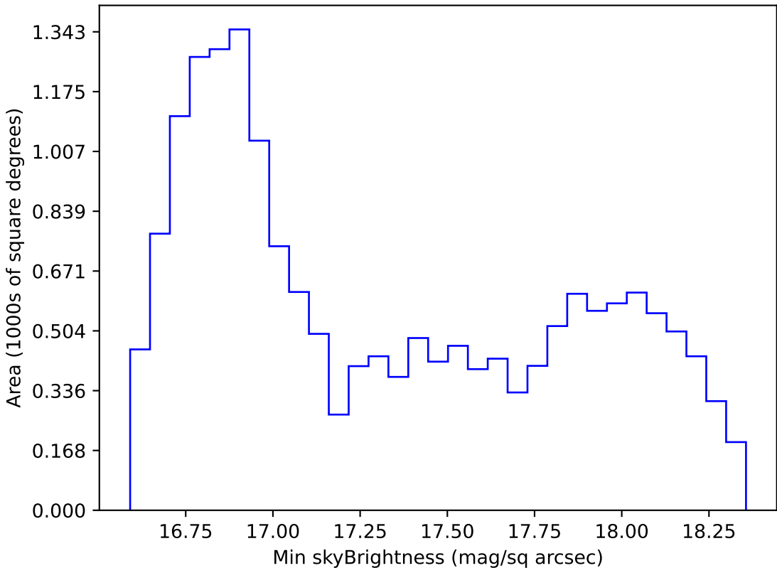
too_elab_r16_d2_giz_v3.4_10yrs WFD z band: Min skyBrightness
