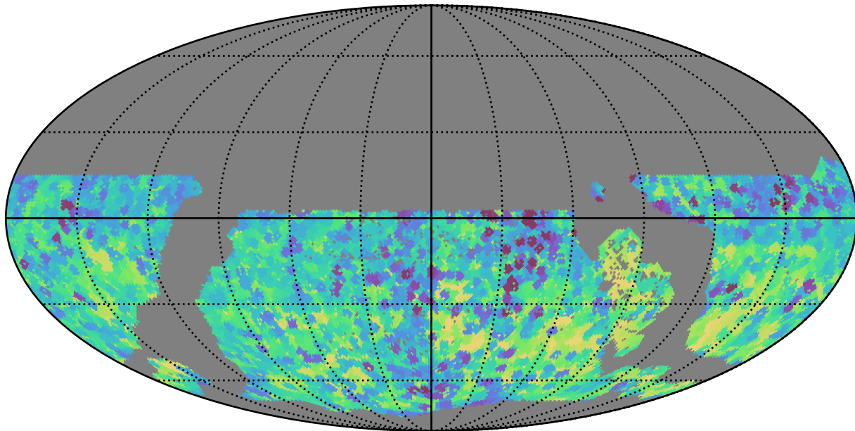
too_elab_r16_d2_giz_v3.4_10yrs WFD y band: Min skyBrightness
