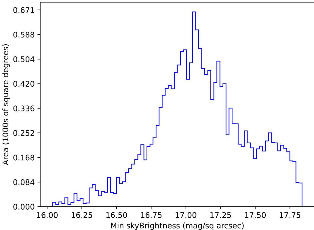
too_elab_r16_d2_giz_v3.4_10yrs WFD y band: Min skyBrightness
