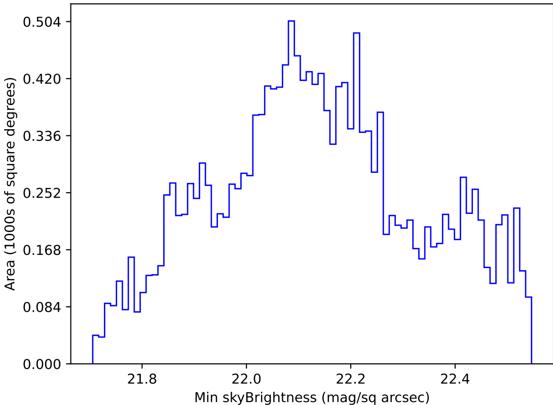
too_elab_r16_d2_giz_v3.4_10yrs WFD u band: Min skyBrightness
