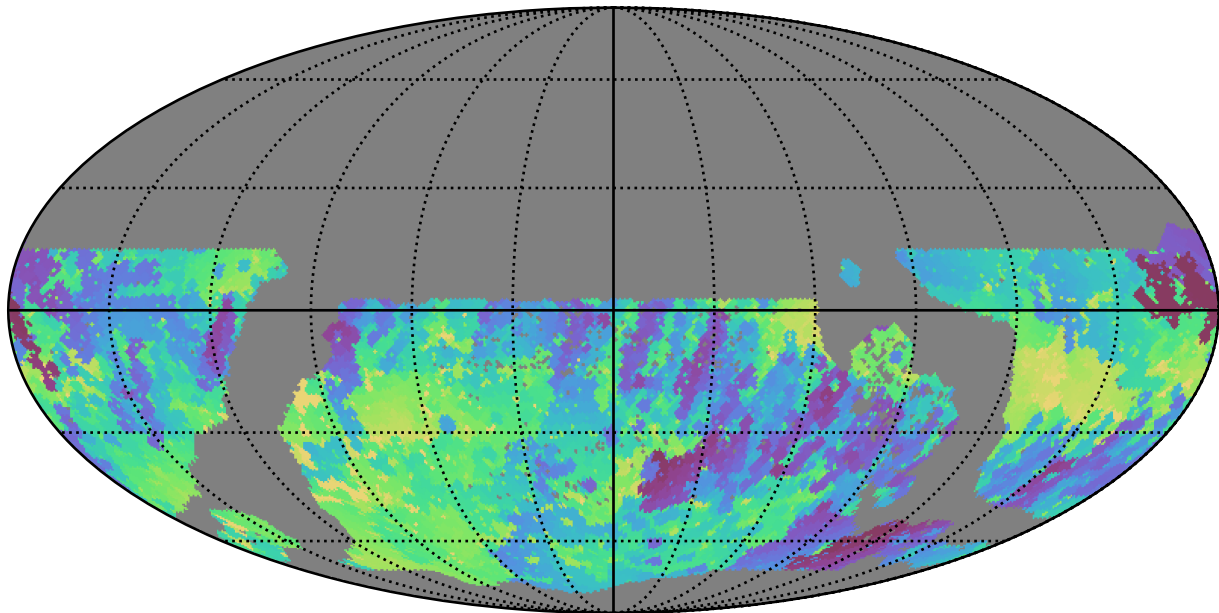
too_elab_r16_d2_giz_v3.4_10yrs WFD r band: Min skyBrightness
