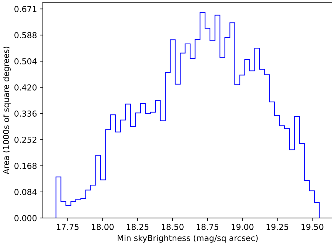
too_elab_r16_d2_giz_v3.4_10yrs WFD r band: Min skyBrightness
