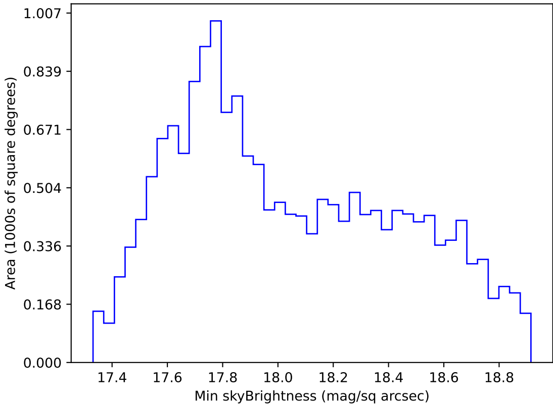
too_elab_r16_d2_giz_v3.4_10yrs WFD i band: Min skyBrightness
