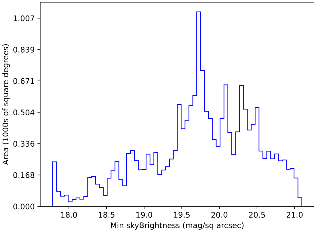
too_elab_r16_d2_giz_v3.4_10yrs WFD g band: Min skyBrightness
