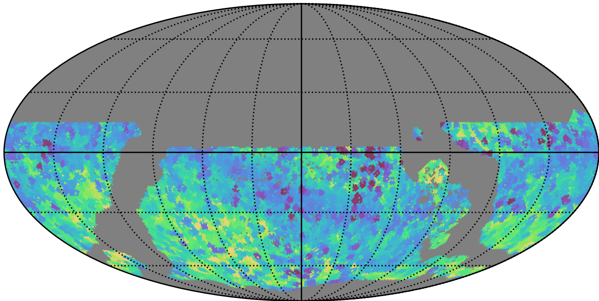
too_elab_r16_d2_giz_v3.4_10yrs WFD all bands: Min skyBrightness
