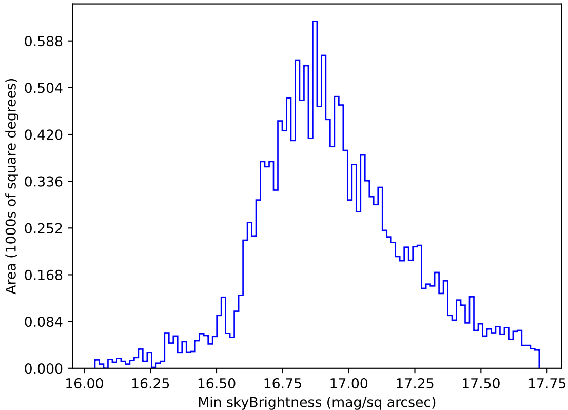
too_elab_r16_d2_giz_v3.4_10yrs WFD all bands: Min skyBrightness
