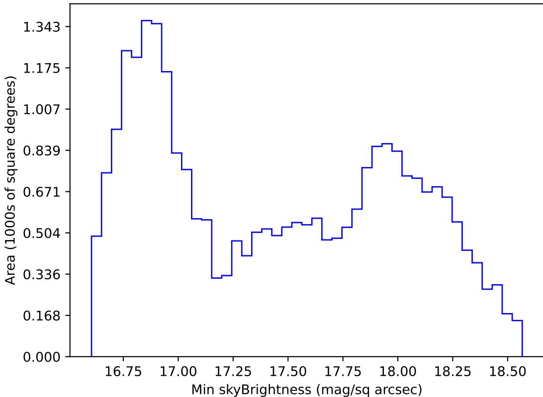
too_elab_r16_d2_giz_v3.4_10yrs All sky z band: Min skyBrightness
