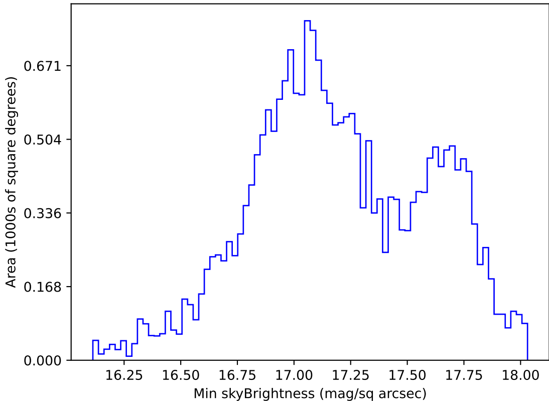
too_elab_r16_d2_giz_v3.4_10yrs All sky y band: Min skyBrightness
