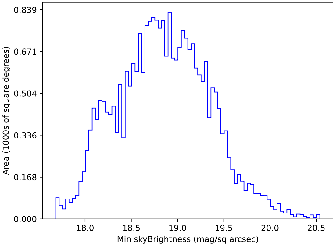
too_elab_r16_d2_giz_v3.4_10yrs All sky r band: Min skyBrightness
