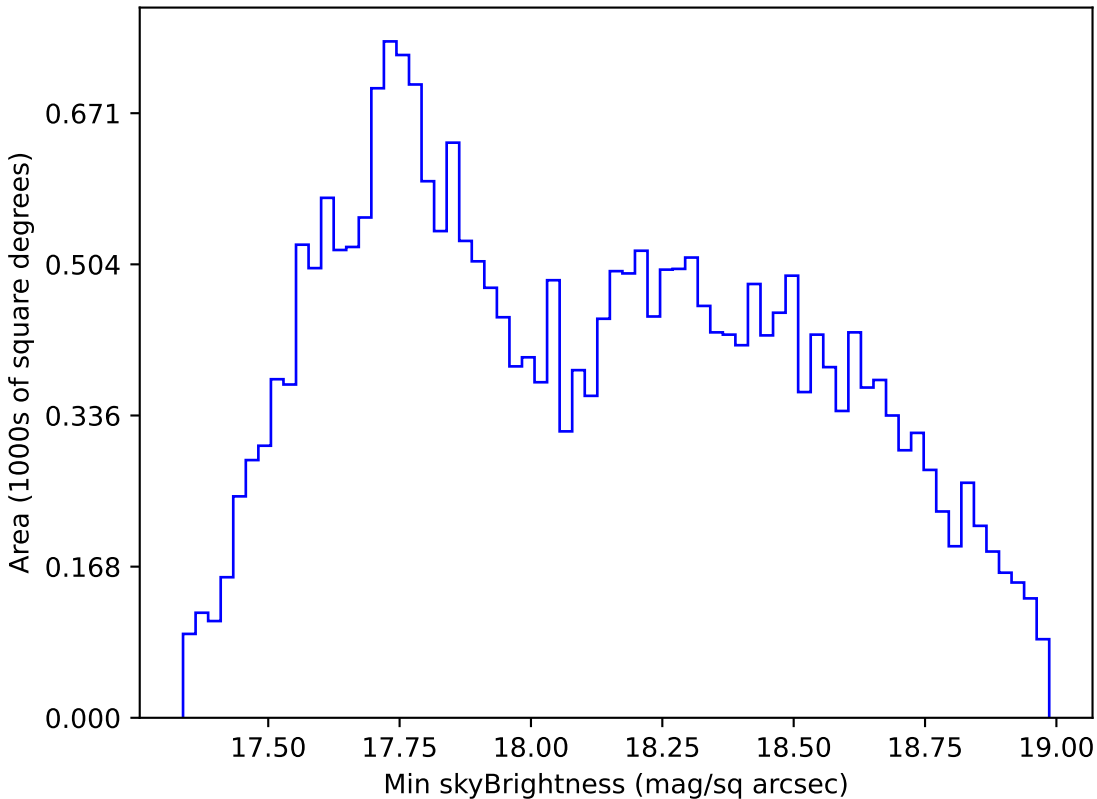
too_elab_r16_d2_giz_v3.4_10yrs All sky i band: Min skyBrightness
