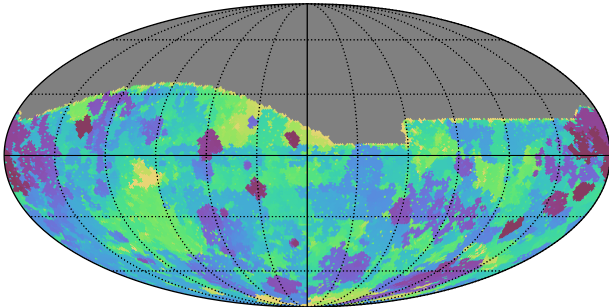
too_elab_r16_d2_giz_v3.4_10yrs All sky g band: Min skyBrightness
