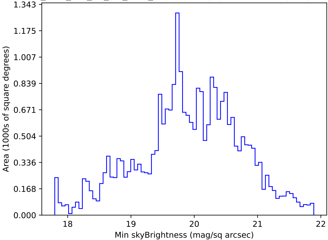
too_elab_r16_d2_giz_v3.4_10yrs All sky g band: Min skyBrightness
