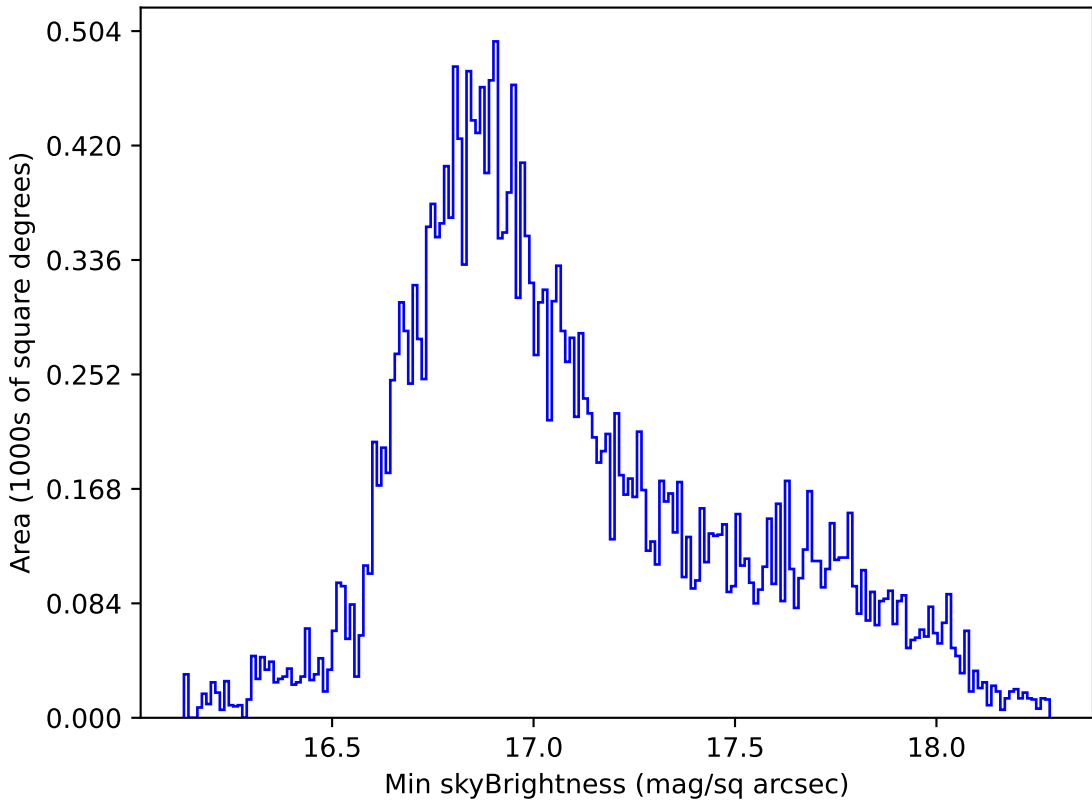
too_elab_r16_d2_giz_v3.4_10yrs All sky all bands: Min skyBrightness
