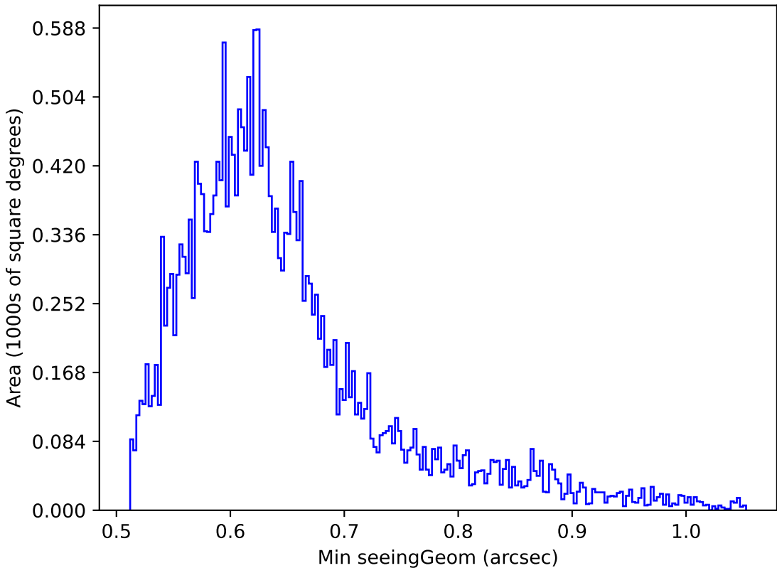
too_elab_r16_d2_giz_v3.4_10yrs Yr 1 z band: Min seeingGeom
