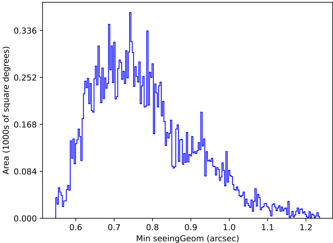
too_elab_r16_d2_giz_v3.4_10yrs Yr 1 u band: Min seeingGeom
