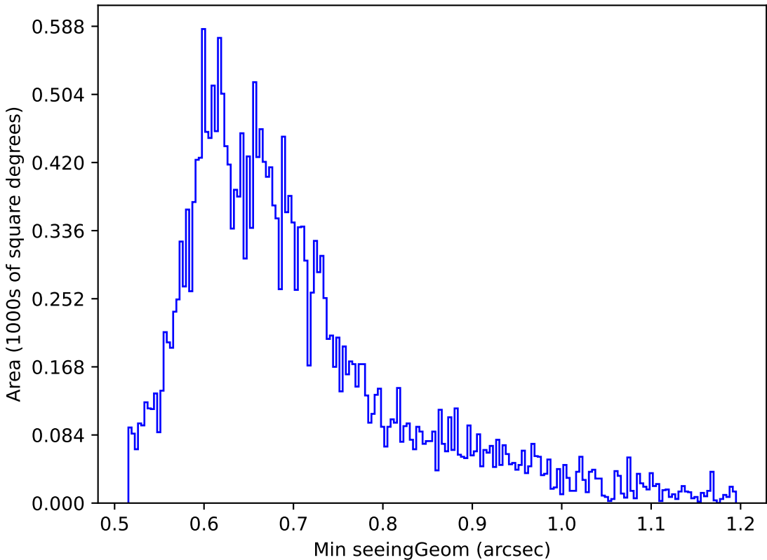
too_elab_r16_d2_giz_v3.4_10yrs Yr 1 g band: Min seeingGeom
