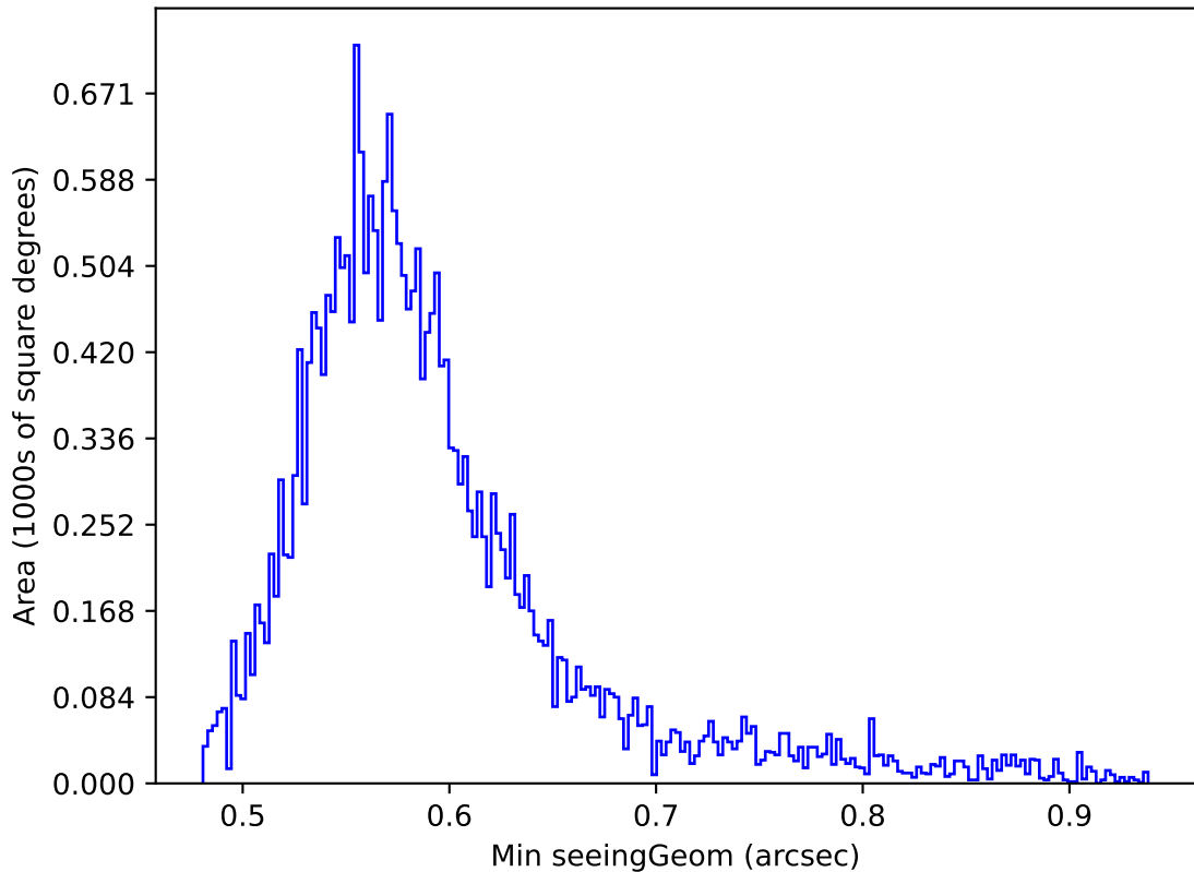
too_elab_r16_d2_giz_v3.4_10yrs Yr 1 all bands: Min seeingGeom
