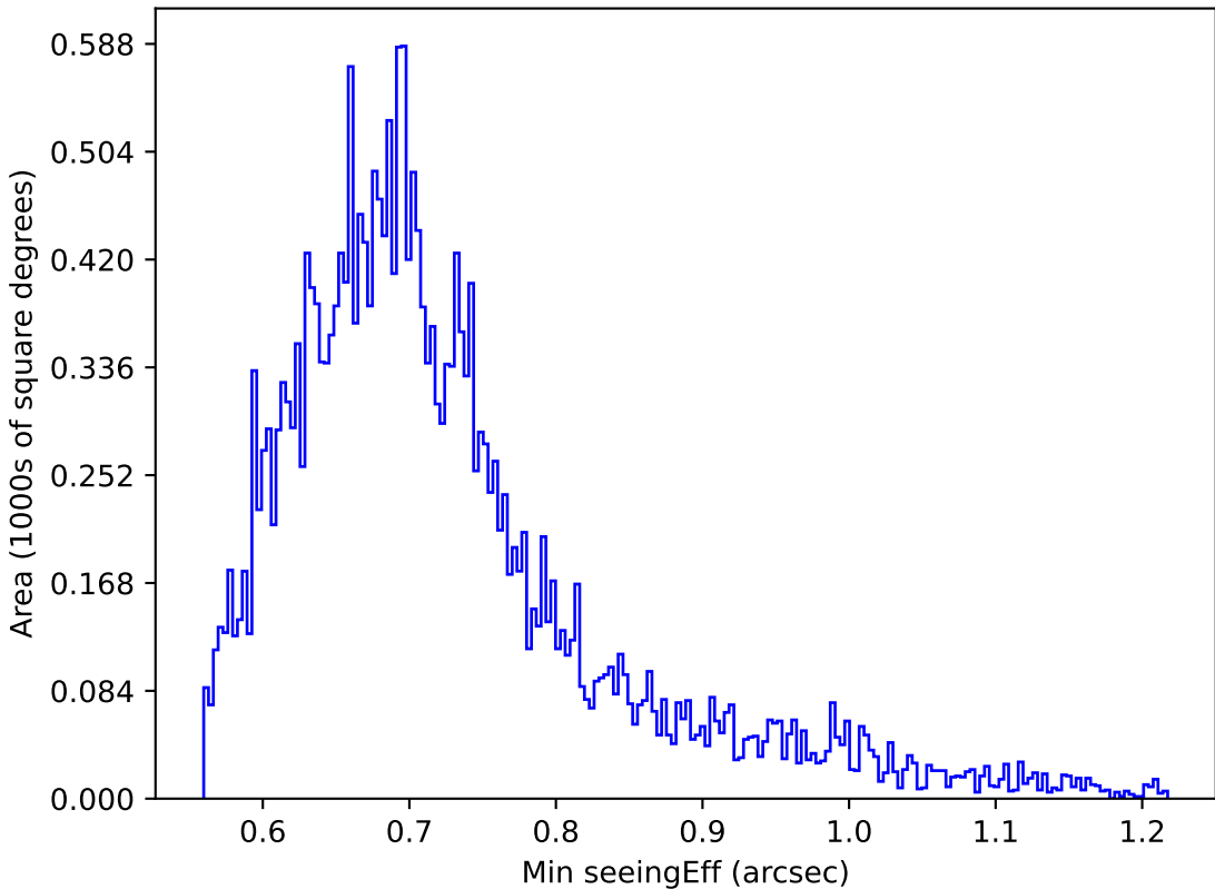
too_elab_r16_d2_giz_v3.4_10yrs Yr 1 z band: Min seeingEff
