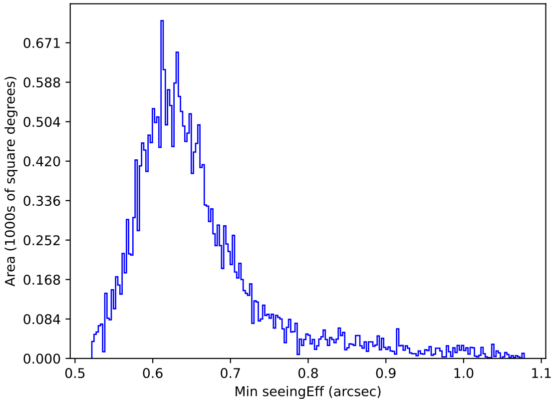
too_elab_r16_d2_giz_v3.4_10yrs Yr 1 all bands: Min seeingEff
