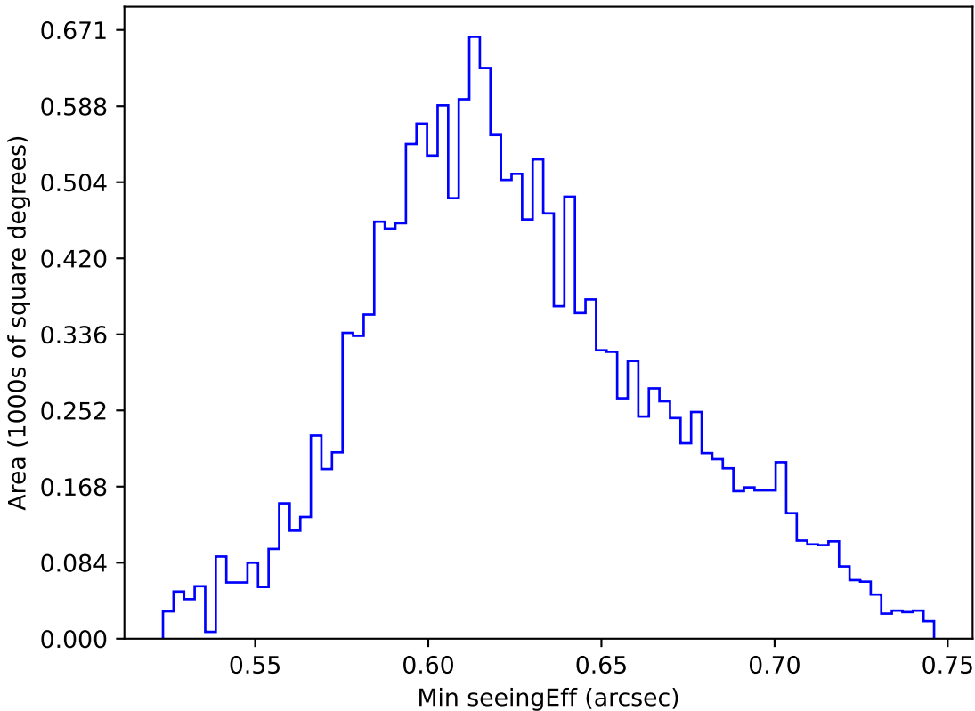
too_elab_r16_d2_giz_v3.4_10yrs WFD y band: Min seeingEff
