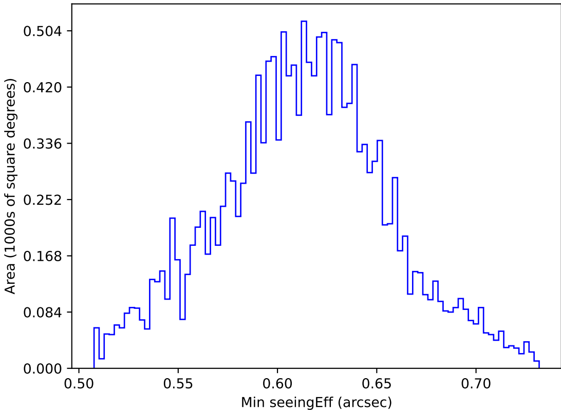
too_elab_r16_d2_giz_v3.4_10yrs WFD r band: Min seeingEff
